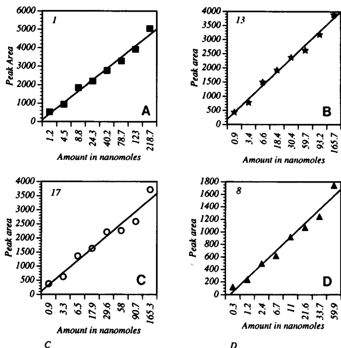
FIG. 3. Quantification of oligosaccharides by peak areas. (A) Disaccharide 1: r^2 = 0.983 . (B) Tetrasaccharide 13: r^2 = 0.990 . (C) Hexasaccharide 17: r^2 = 0.955 . (D) Disaccharide 8: r^2 = 0.972 .
