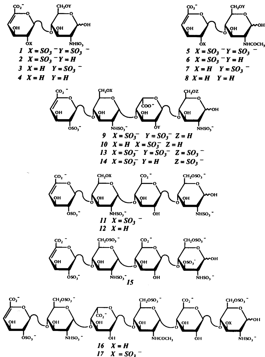
FIG. 1. Structures of heparin-derived disaccharides and oligosaccharides 1-17.
