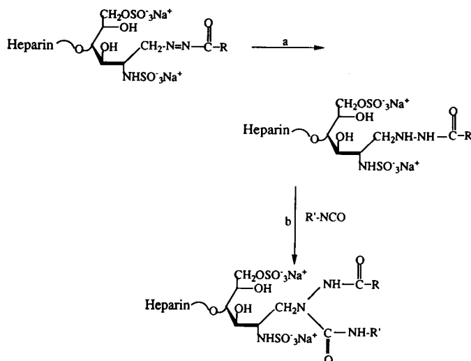
Scheme 3 —Synthetic scheme for the coupling of two alkyl chains to heparin. Step a is performed on the heparin hydrazone derivative when R is C 12 in 20% aqueous methanol with H 2 over Pd/C. Step b is performed in methylene chloride on the tetrabutylammonium salt of heparin when R is C 18 .
