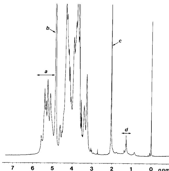
Figure 2 —The 500-MHz 1 H-NMR spectrum of the (C 12 ) lauryl hydrazide derivative of heparin. The signals are labeled as follows: a, corresponding to the anomeric protons of heparin; b, corresponding to HO 2 H; c, corresponding to N-acetyl (CH 3 ); and d, corresponding to the methylene signals of the lauryl chain.
