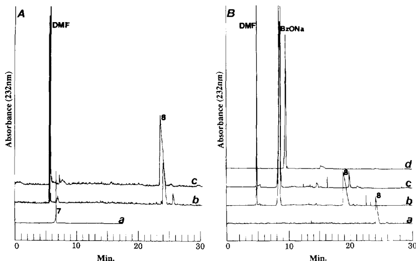
Fig. 2. Electropherograms of: A, sulfation of 6- O -benzoyl sucrose 7 , \text{SO}_3 \cdot \text{NMe}_3 , \text{Me}_2\text{NCHO} , 50^\circ\text{C} (a, 0 h; b, 0.5 h; c, 1 h); B, debenzoylation of 8 , \text{NaOH} , \text{Me}_2\text{NCHO} , 4^\circ\text{C} , (a, purified 8 ; b, 1 h; c, 9 h; d, 18 h).
