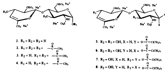
Fig. 1. Structures of heparin disaccharide derivatives.
