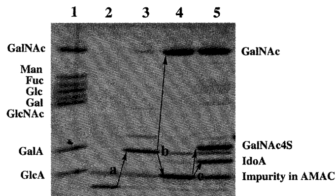
Figure 3. Polyacrylamide gel electrophoresis of oligosaccharides fluorescently labeled with AMAC. Lane 1 contains a mixture of monosaccharide standards; Lane 2 contains disulfated trisaccharide; Lane 3 contains disulfated trisaccharide treated with (a) arylsulfatase B (the monosulfated trisaccharide product ran just below the GalA standard); Lane 4 contains disulfated trisaccharide treated with (a) arylsulfatase B and (b) N -acetyl hexosaminidase (the monosulfated disaccharide product runs at the same position as a contaminant present in the AMAC label seen in lanes 2–5); and Lane 5 contains disulfated trisaccharide treated with (a) arylsulfatase B, (b) N -acetylhexosaminidase and (c) \alpha -L-iduronidase.
