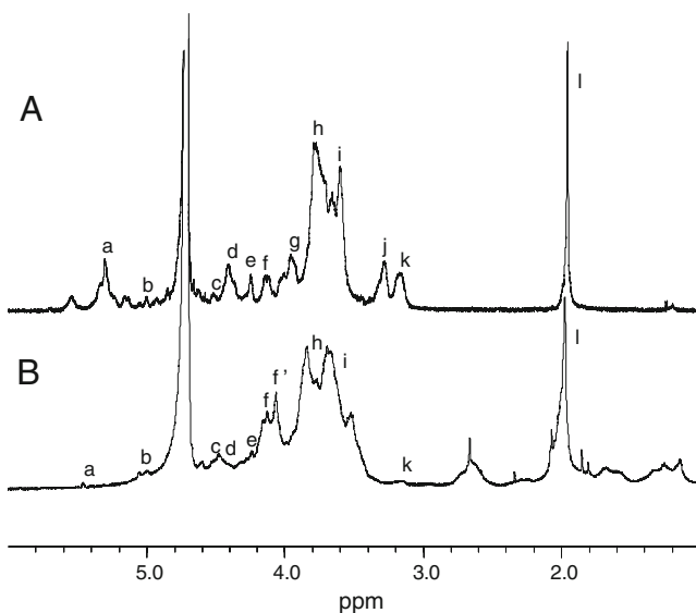
Fig. 4 1D- ^1 H-NMR spectra of HS samples. A ^1 H-NMR of standard heparan sulfate obtained from porcine intestine; B ^1 H-NMR of heparan sulfate from adult fish. a H-1 GlcNAc; b H-1 IdoA2S; c H-5 IdoA2S; d H-1 GlcA; e H-2 IdoA2S; f H-3 IdoA2S and H-6 GlcNS6S or GlcNAc6S; f' H-4 IdoA2S; g and h H-2 and H-3 GlcNAc, H-6 and H-5 GlcNS or GlcNAc; i H-3 and H-4 GlcNS, GlcNAc, GlcNS6S or GlcNAc6S; j H-2 GlcA; k H-2 GlcNS or GlcNS6S; l CH 3 of acetyl group
