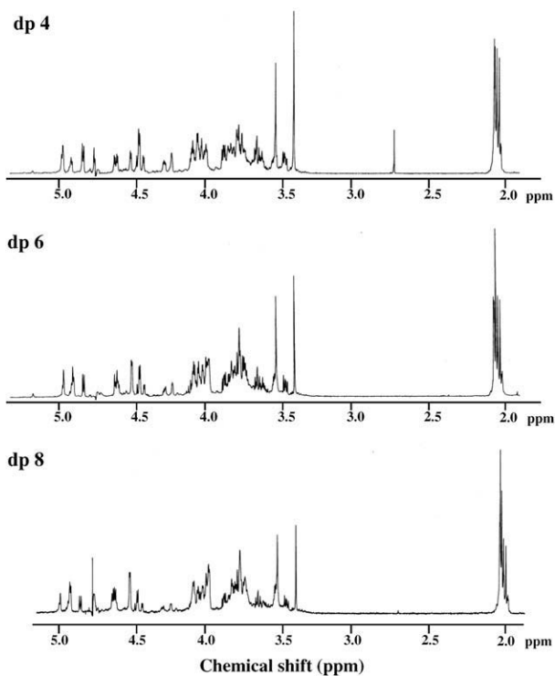
Figure 6. ^1\text{H} NMR spectra of the purified oligosaccharides obtained from dermatan sulfate by solvolysis.
