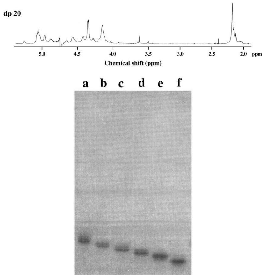
Figure 7. Gradient PAGE profile of per-O-sulfonated chondroitin oligosaccharides. Lanes; a, per-O-sulfonated dp 20; b, per-O-sulfonated dp 18; c, per-O-sulfonated dp 16; d, O-sulfonated dp 14; e, per-O-sulfonated dp 12; f, per-O-sulfonated dp 10. Stained by Alcian Blue.
