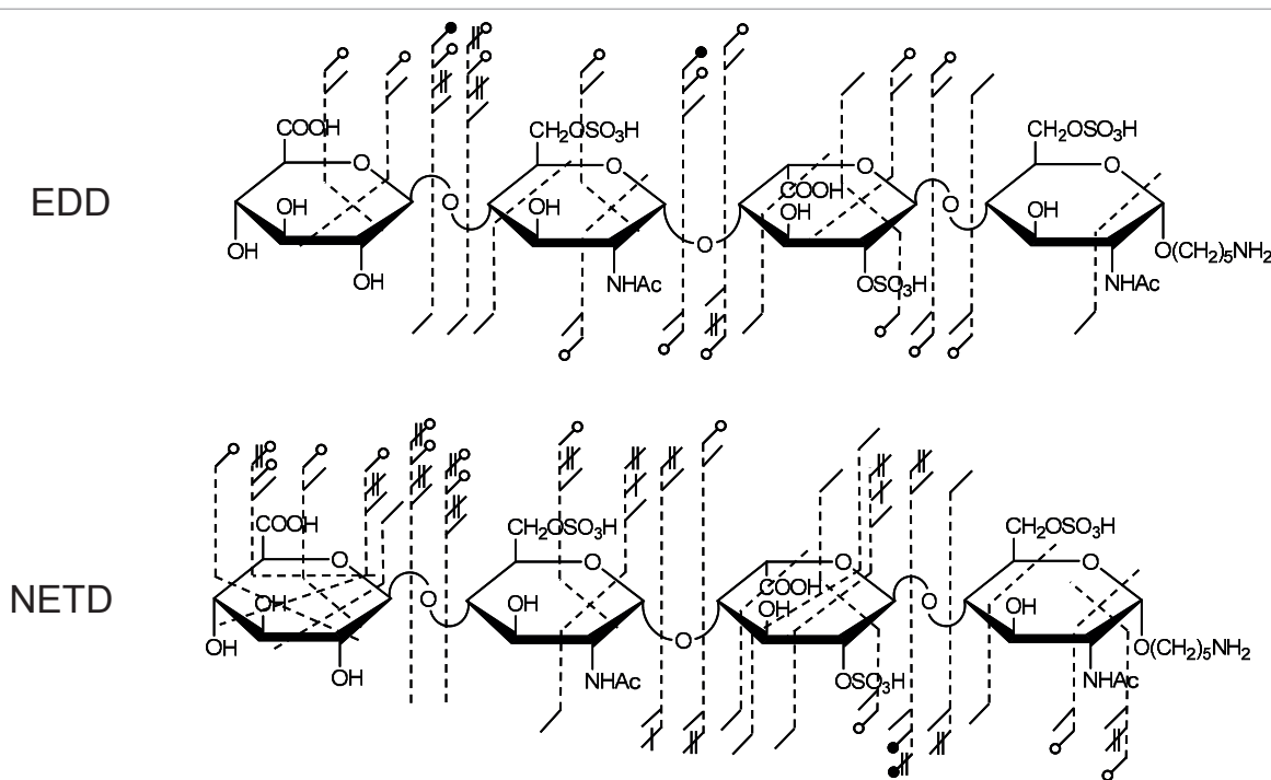
Figure 3. Comparison of the product ion distributions generated by EDD and NETD for HS2.
