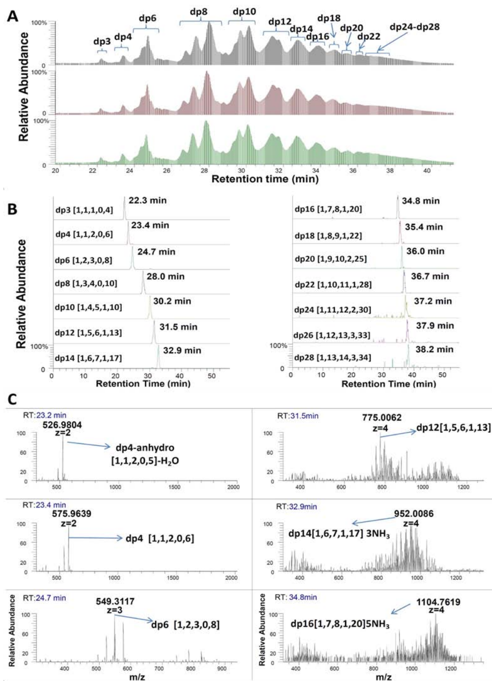
Figure 2. (A) Total ion chromatogram TIC of intact LMWH (triplicate) using ESI HILIC LC-FT MS. Heparin oligomer dp3–dp28 can be separated and FT MS resolved by HILIC LC MS corresponded to the size and charge. (B) Selected extracted ion chromatograms (EIC) for the major LMWH structures from dp3 to dp28 demonstrated the highly efficient separation of LMWH and sensitive detection using this HILIC LC-FT MS platform. (C) Selected mass spectra and identified major structures. Table 1S in the Supporting Information showed the detailed identification information.
