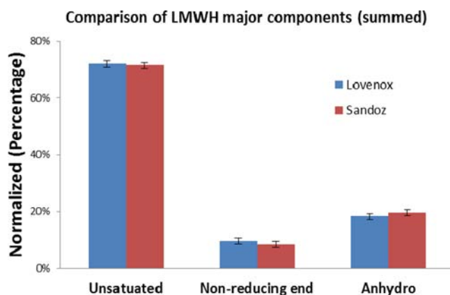
Figure 5. Relative amount (percentage) of identified 3 major LMWH components.
