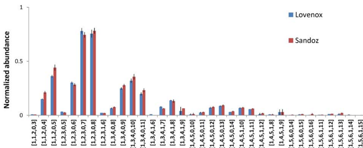
Figure 3. Quantitative comparison of identified anhydro-heparin oligosaccharides from two commercialized LMWH products. Oligosaccharide compositions are given as [ \Delta HexA, HexA, GlcN, Ac, SO 3 ].
