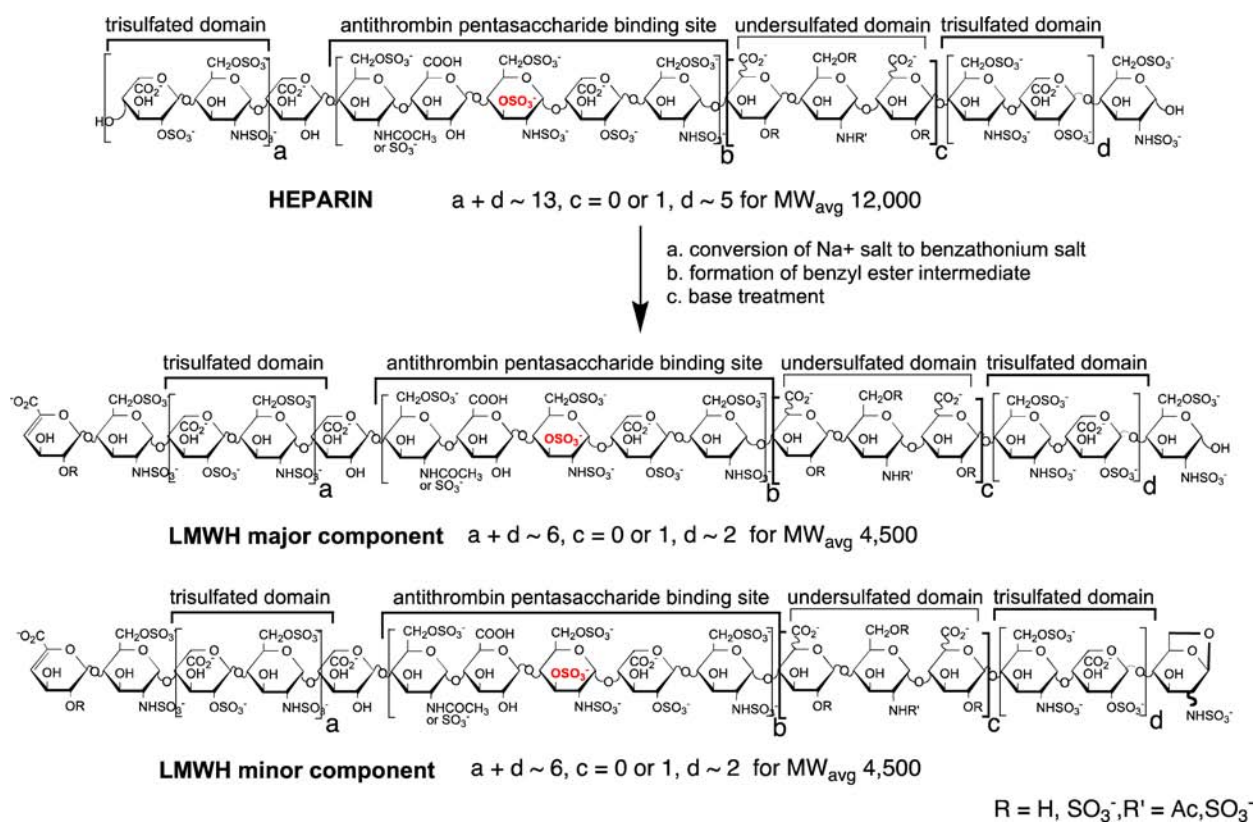
Figure 1. Synthesis and structure of LMWH (enoxaparin). It is produced by optimized cleavage of the of heparin from porcine intestinal mucosa and is converted to its benzathonium salt, and then to its benzyl ester, and is chemically \beta -eliminated by alkaline treatment affording enoxaparin as a sodium salt with a mean molecular weight of 4000–4500 Da with approximately 90% of the oligosaccharides within the range 2000–8000 Da. The structures of a major and a minor enoxaparin chain are shown.
