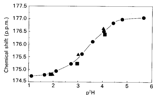
Fig. 5. Determination of the \text{p}K_a of uronic acid residues in heparin
