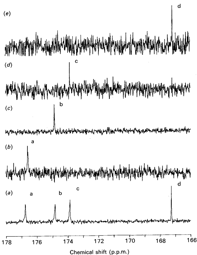
Fig. 2. Selective INEPT experiment performed on hexasaccharide (V) at 106 mM; p^2\text{H} (measured) 0.90
