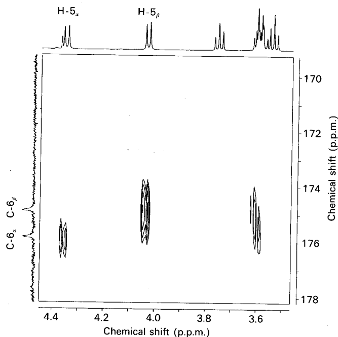
Fig. 1. HMBC spectrum of D-glucopyranosyluronic acid (II)
